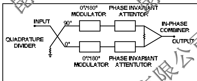
FIGURE 1 I-Q Vector Modulator Block diagram
