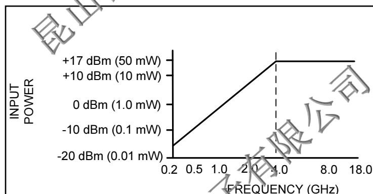
Fig. 3-Model 3250A, maximum peak and average operating power without performance degradation
