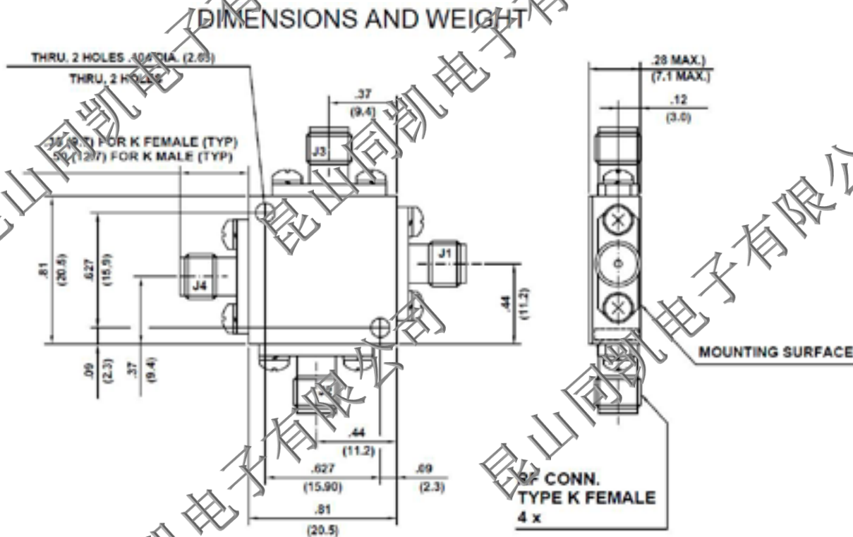
MODEL 7050 Wt: 1 oz (28gr) approx.
