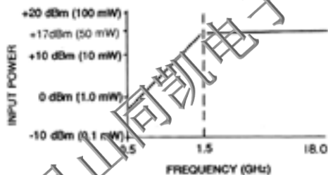
Fig. 3- Series 346C, maximum peak and average operating power without performance degradation
