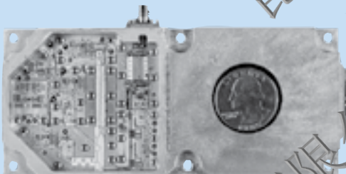
Fig. 1 - Multi-Band DTO (RF side view)
