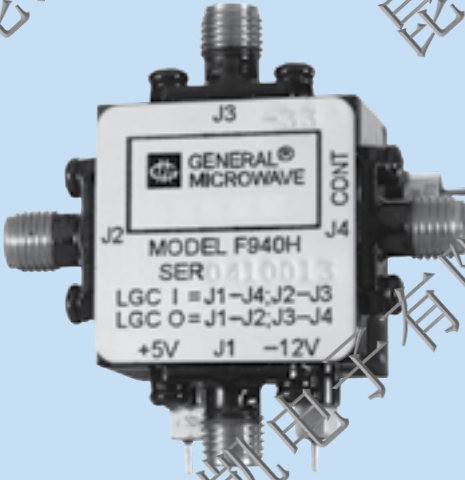
Switch Model F940H
